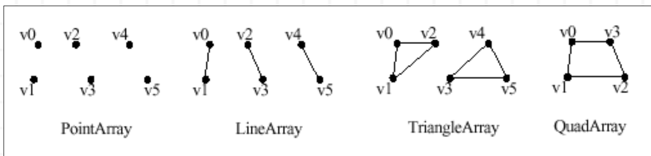
Figura 2-13. Subclases de GeometryArray.
