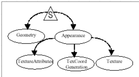
Figura 7-18, Manajo de Appearance con Texture, TextureAttributes, y TexCoordGeneration.
